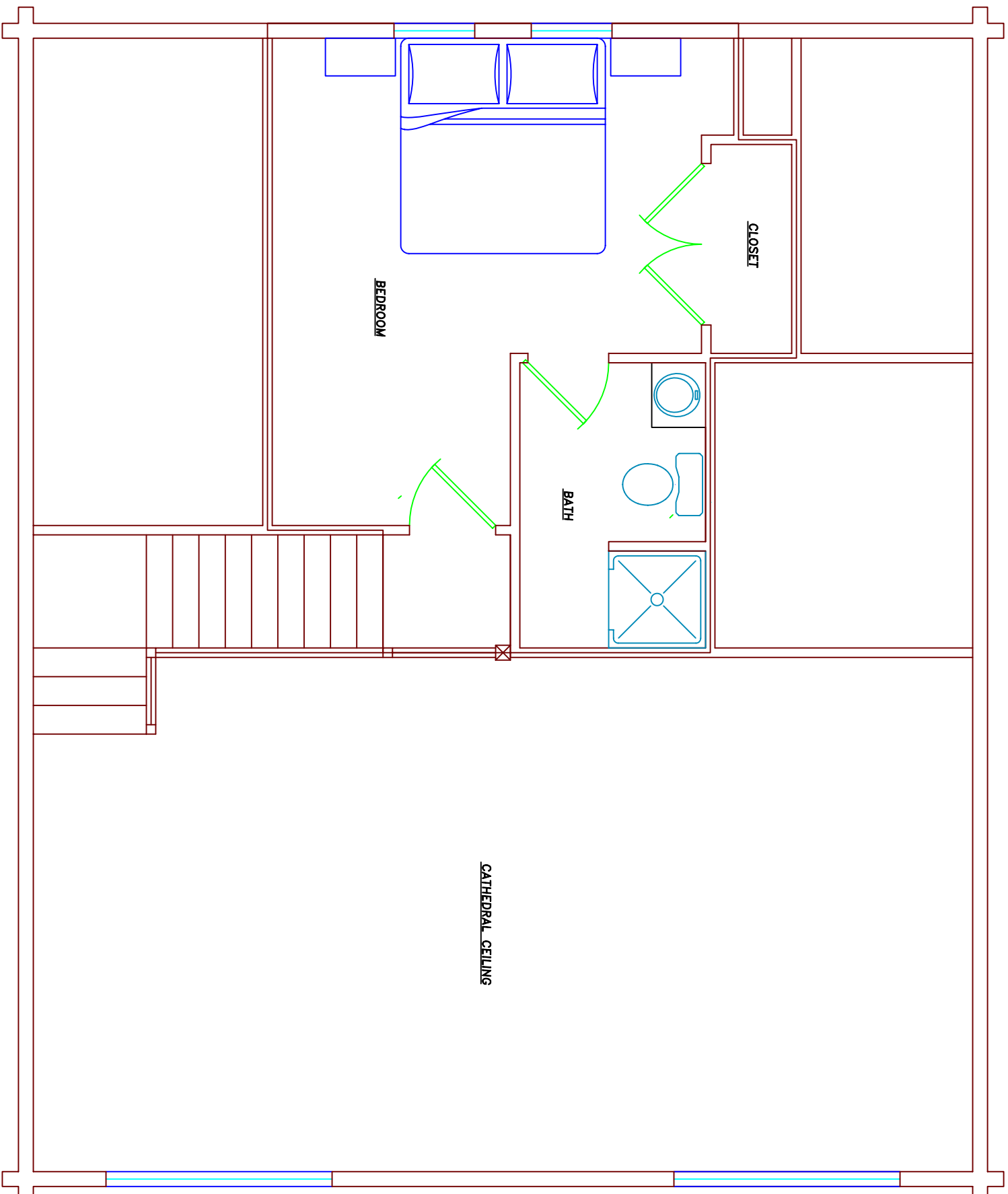
CABIN "F" SECOND FLOOR PLAN (10)
