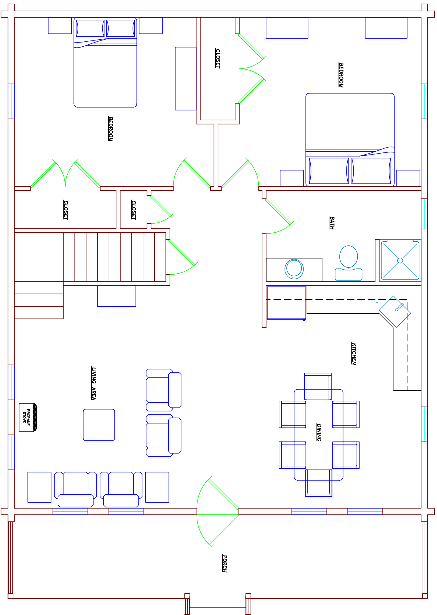
CABIN "F" FIRST FLOOR PLAN (10)
